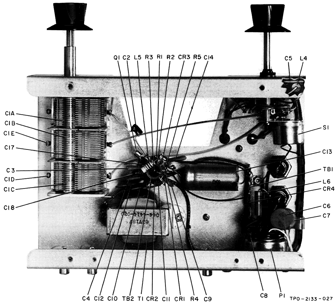
Figure 4-2. 55G-1 Component Identification (Sheet 2 of 2).
