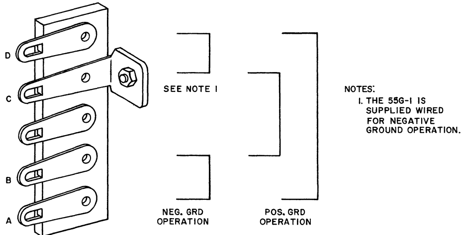
Figure 1-3. Jumper Connections for Negative or Positive Ground Operation of 55G-1.
